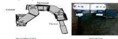
Figure 2. Leg design of robot.
